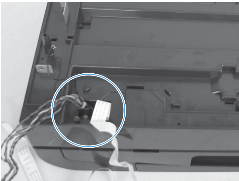
Figure 1-72 Remove the Document feeder whole unit kit and scanner whole unit kit (4 of 6)
